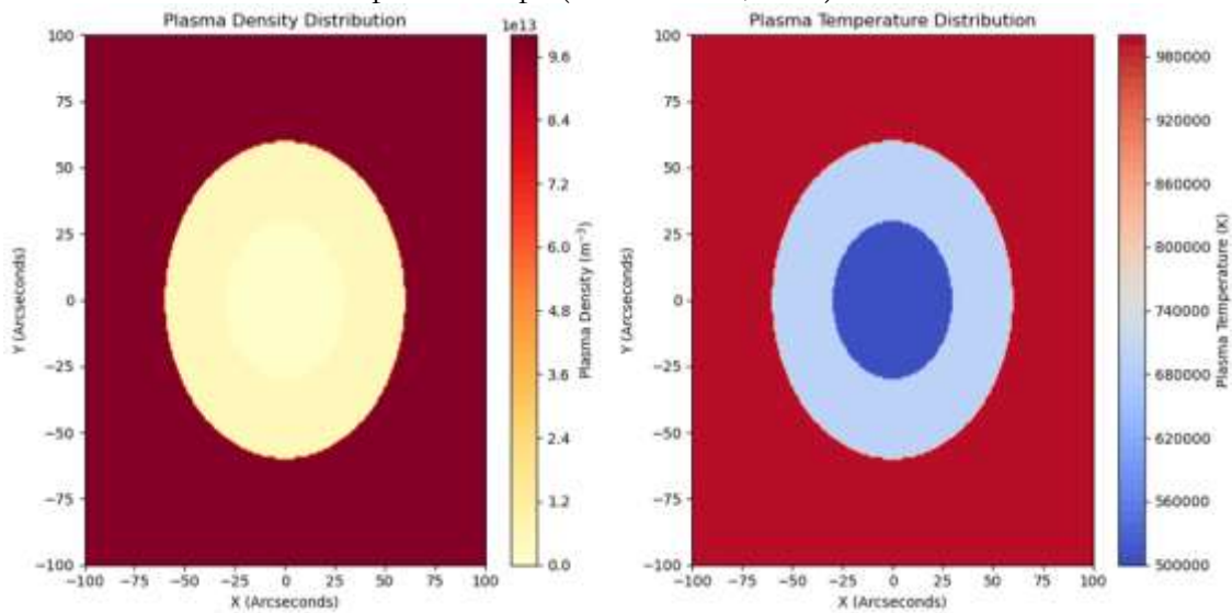
Figure 4. The core and the secondary dimmings of the plasma and temperature distributions
