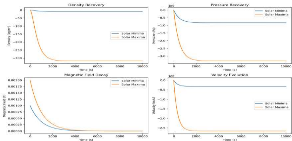
Figure 3. The solar minima and maxim during the recovery of density, pressure, magnetic field, and velocity of evolution
